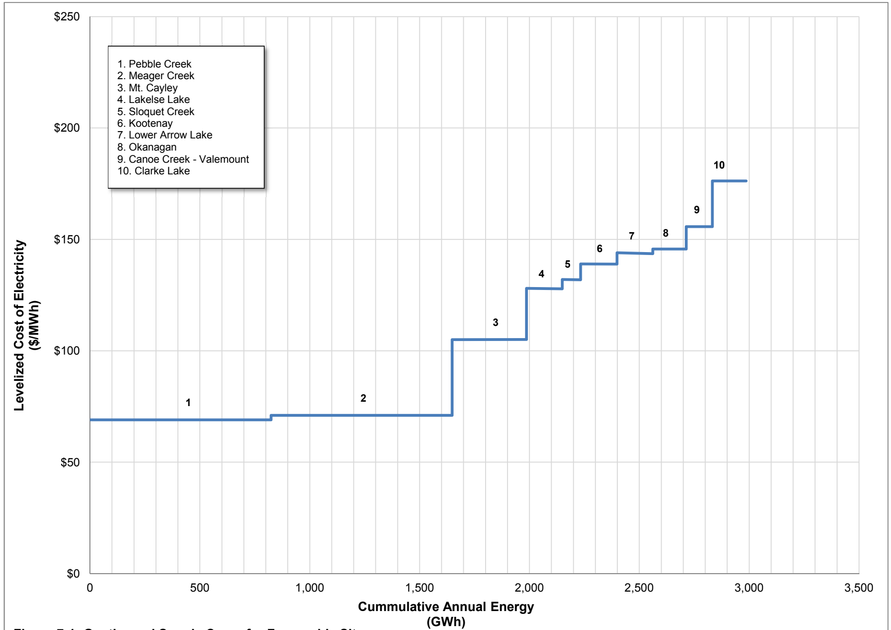
Figure 7-1: Geothermal Supply Curve for Favourable Sites
