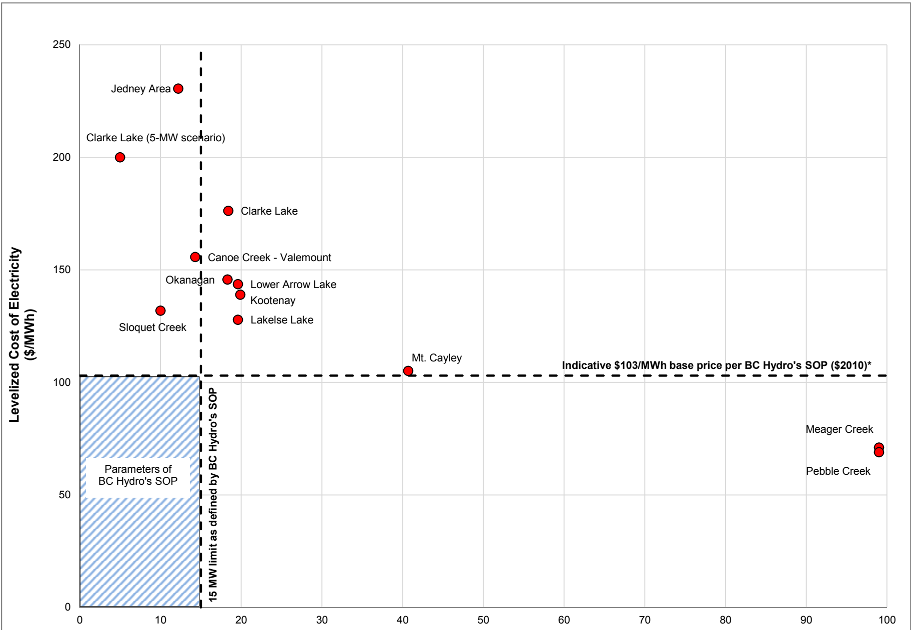
Figure E1-3: Geothermal Resources - LCOE vs Capacity
