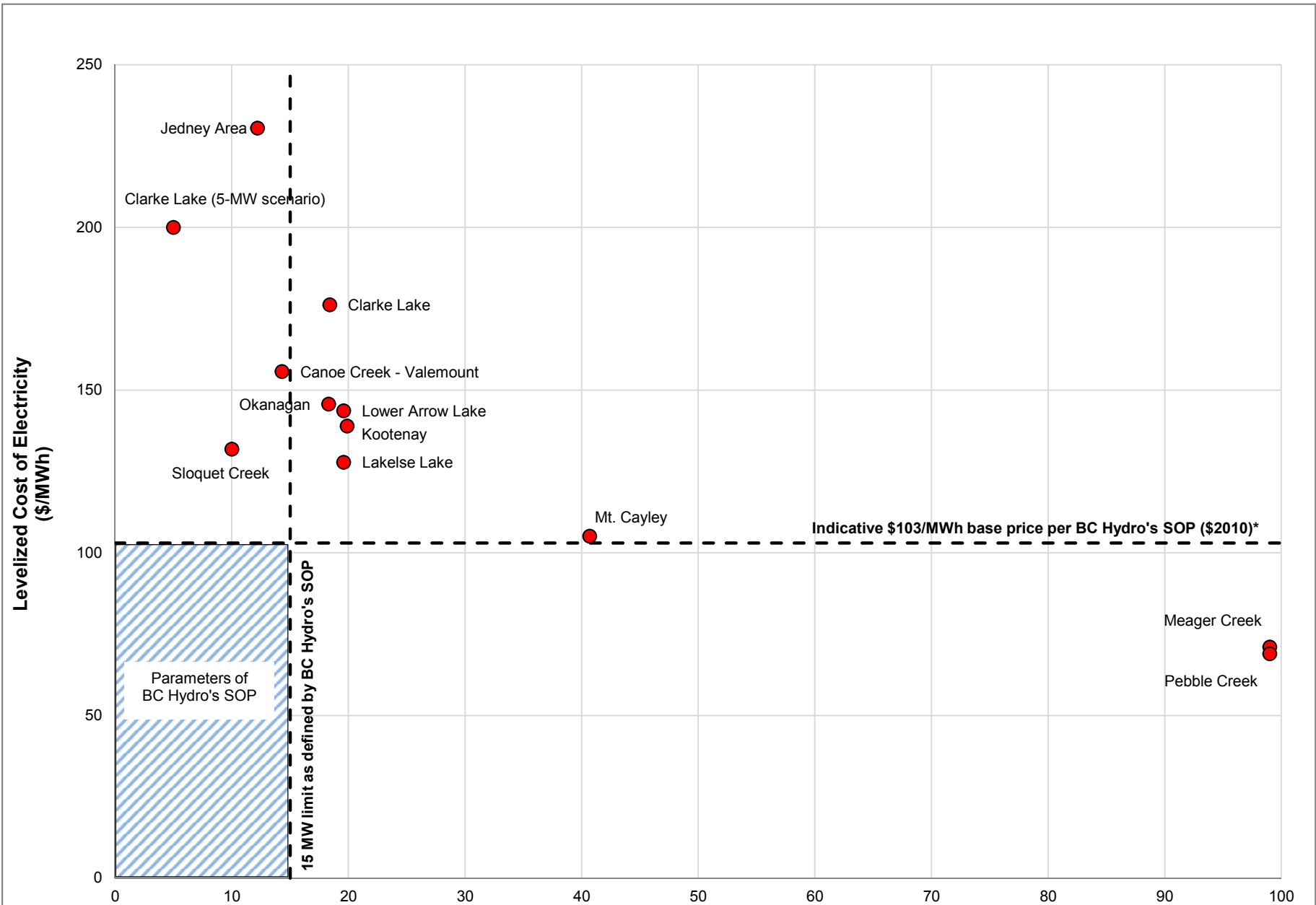
Figure 7-2: Geothermal Resources - LCOE vs Capacity
